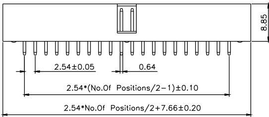
P/N:2316S-XXG
