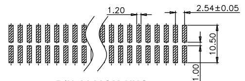
P/N:2316SM-XXG
