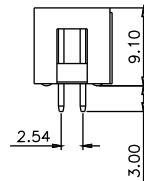
P/N:2316S-XXG
