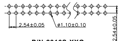
P/N:2316S-XXG P/N:2316R-XXG
